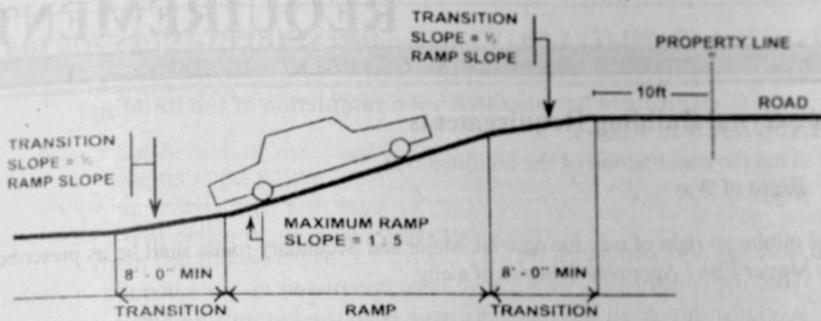
FIG. a RAMP SLOPES TRANSITIONS ARE REQUIRED ONLY IF RAMP SLOPE EXCEEDS 1 : 10
