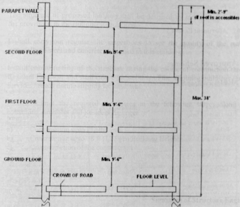
Fig-2.1 Height of Residential Building
