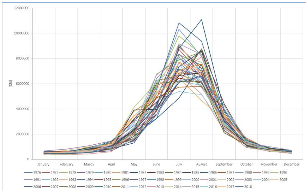
Figure 5-11: Monthly Inflows to Tarbela Reservoir, 1–76 – 2018
