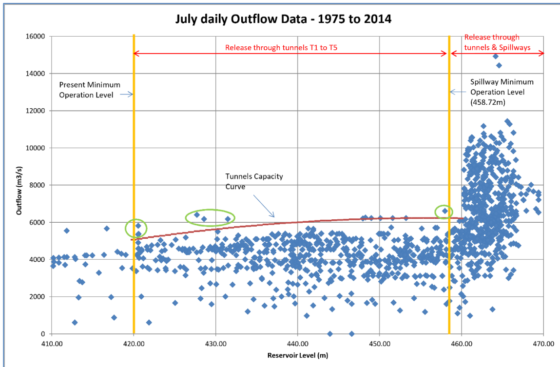
Figure 7-3: Historical Daily Outflows from T5 in the Month of July
