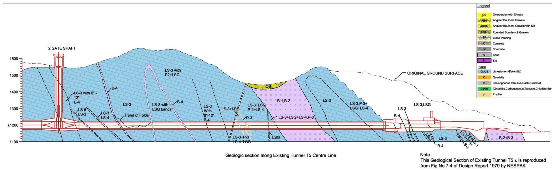
Figure 5-3: Geologic section of Tunnel 5 showing different rock units (reproduced)
