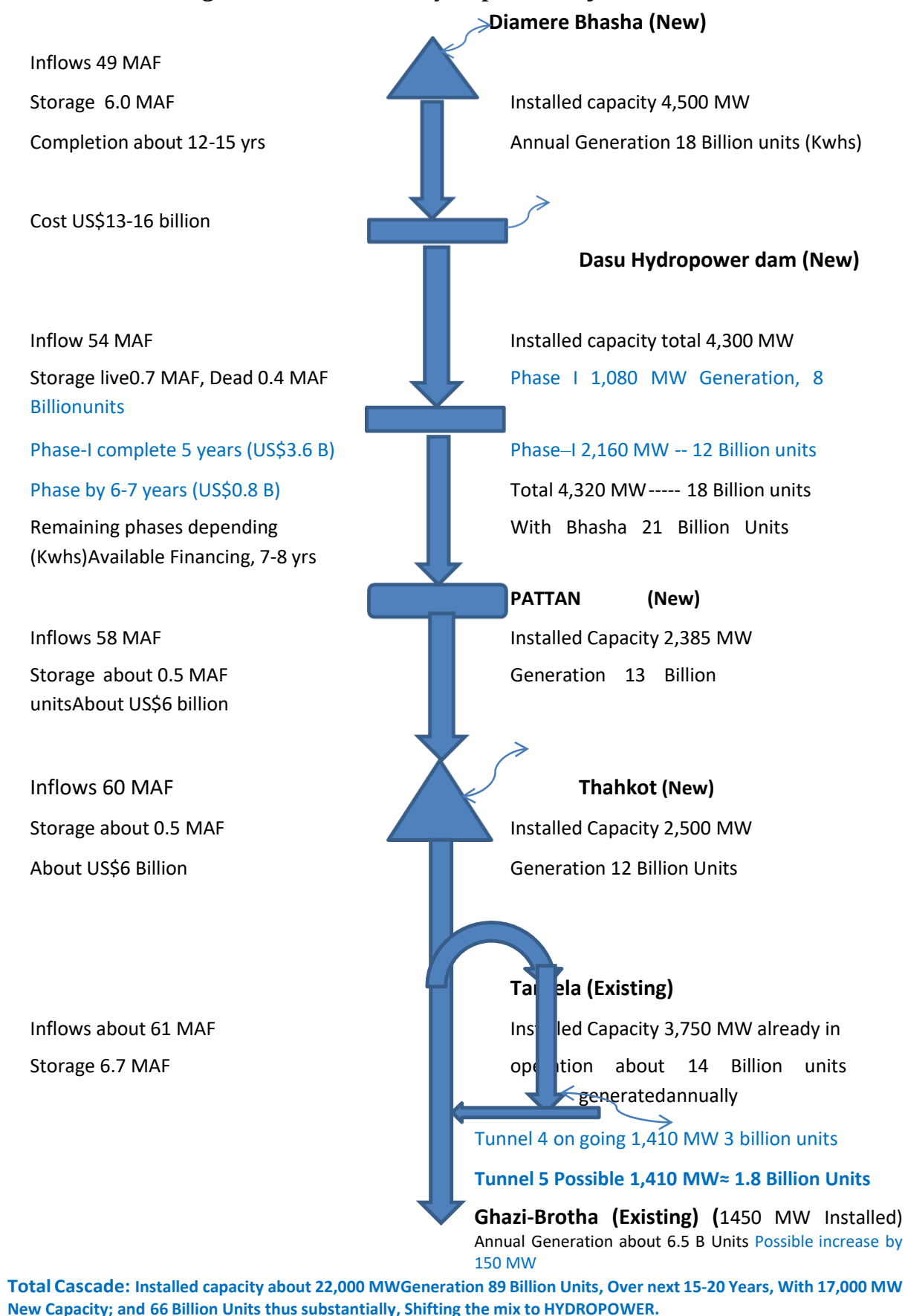
Figure 9-2: Cascade of Hydropower Projects on Indus
