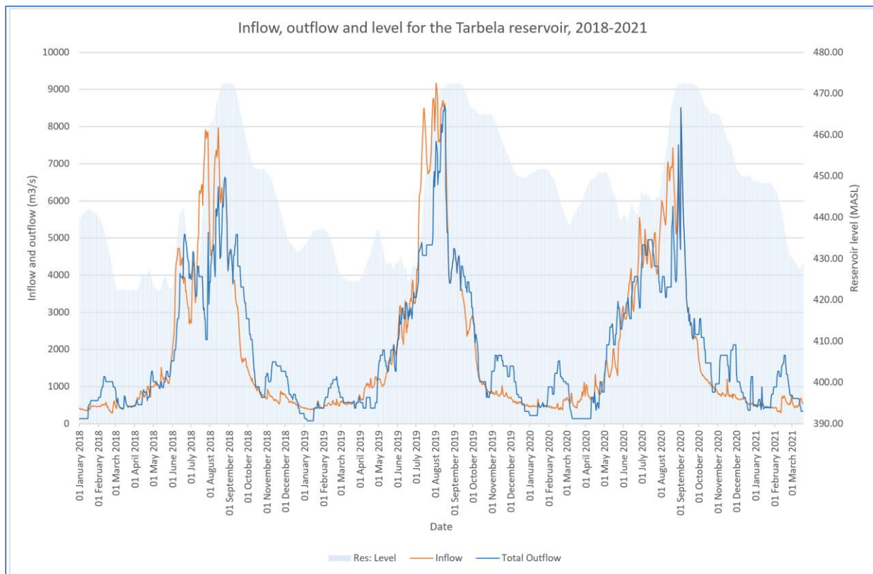
Figure 5-10: Inflow, outflow and reservoir level, 2018-2021
