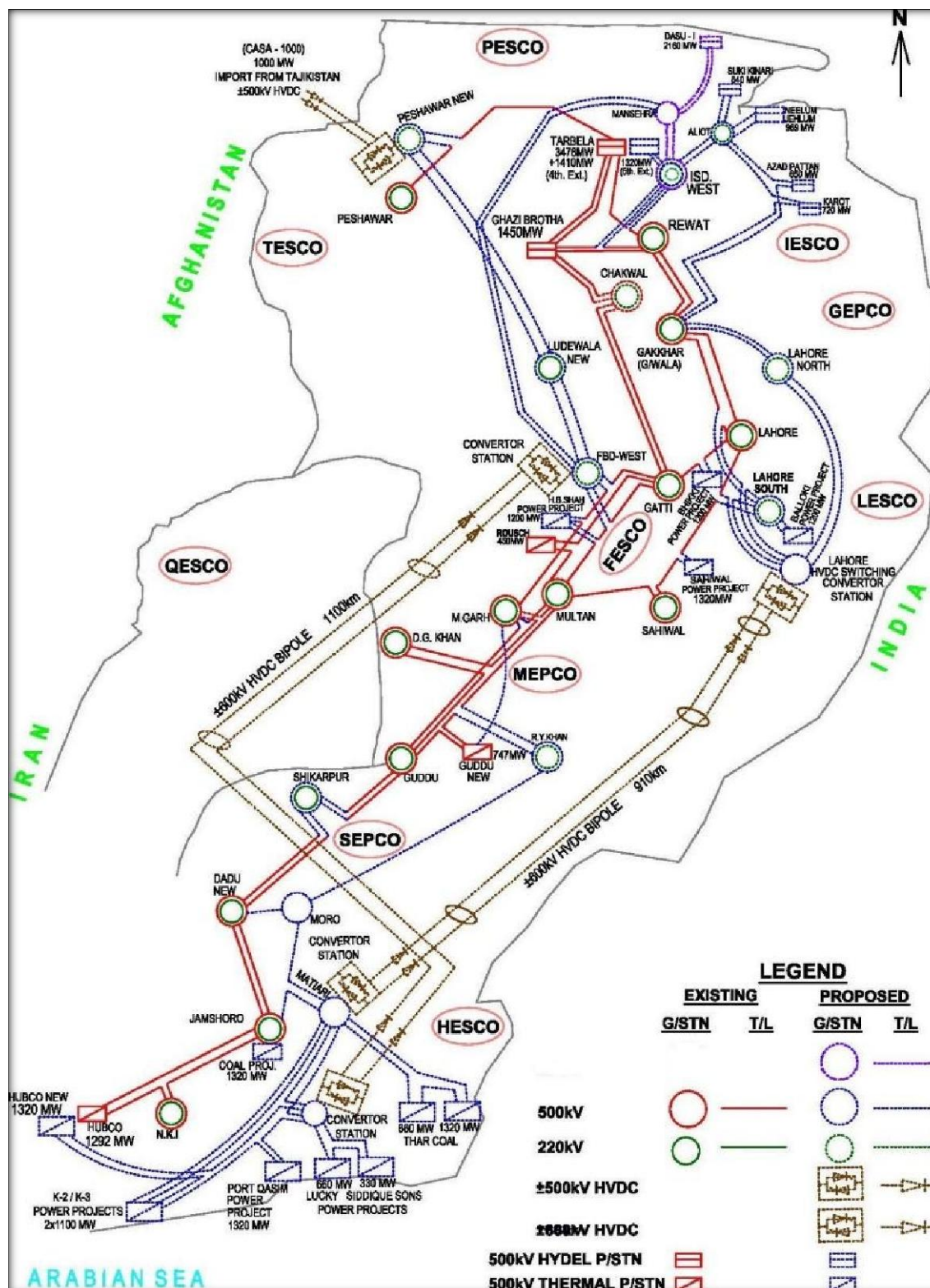
Figure 9-4: Future Planned 500 kV Transmission Line Network in Pakistan (2021-2022)
