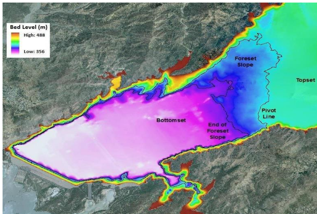
Figure 5-9: Reservoir Bathymetry
