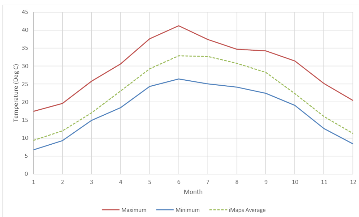
Figure 5-5: Maximum, minimum and mean monthly temperature in the project area (2008-18)
