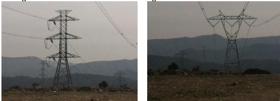
Figure 3-6: Double Circuit Tower and Single Circuit Flat Formation Tower
